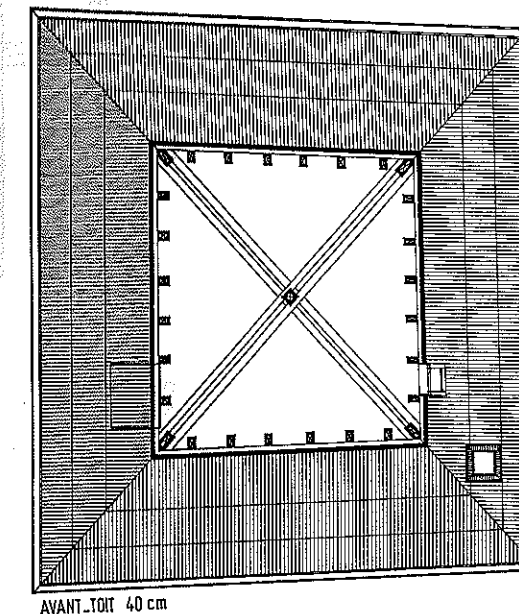
COMBLES
